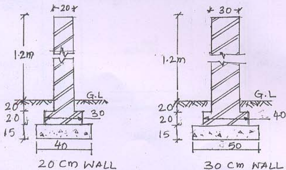
Figure 3(b). Section of a compound walls
