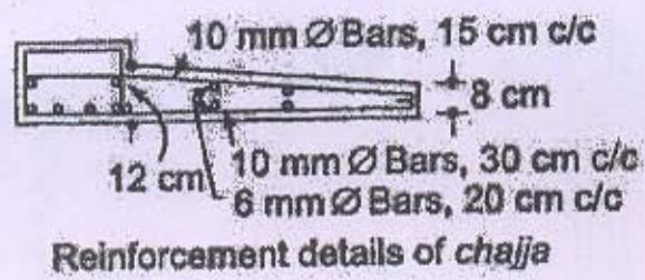
Figure 2. Section of Chajja.
